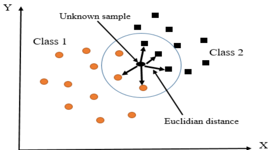
Figure 4: KNN Example Two-class classification [22]
