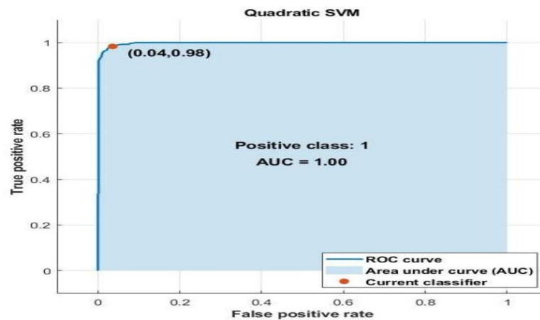
Figure 6: QSVM Classifier Region of Convergence
