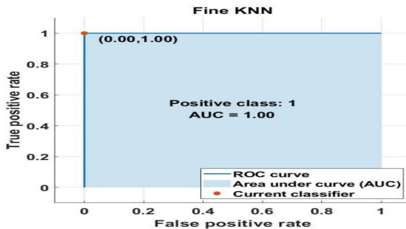
Figure 8: KNN Classifier Region of Convergence
