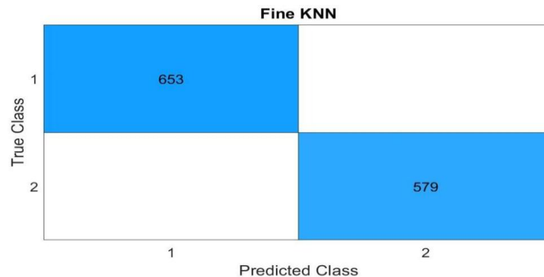
Figure 7: KNN classifier confusion matrix
