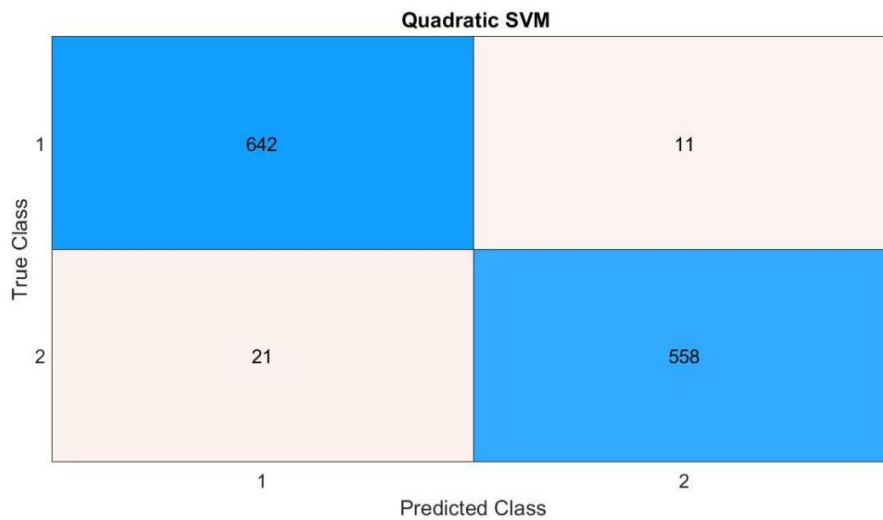
Figure 5: QSVM classifier Confusion matrix
